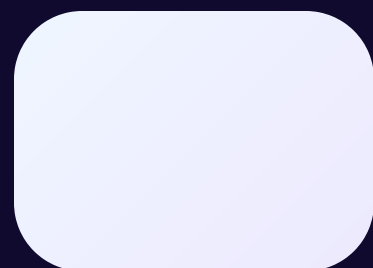
border-radius
